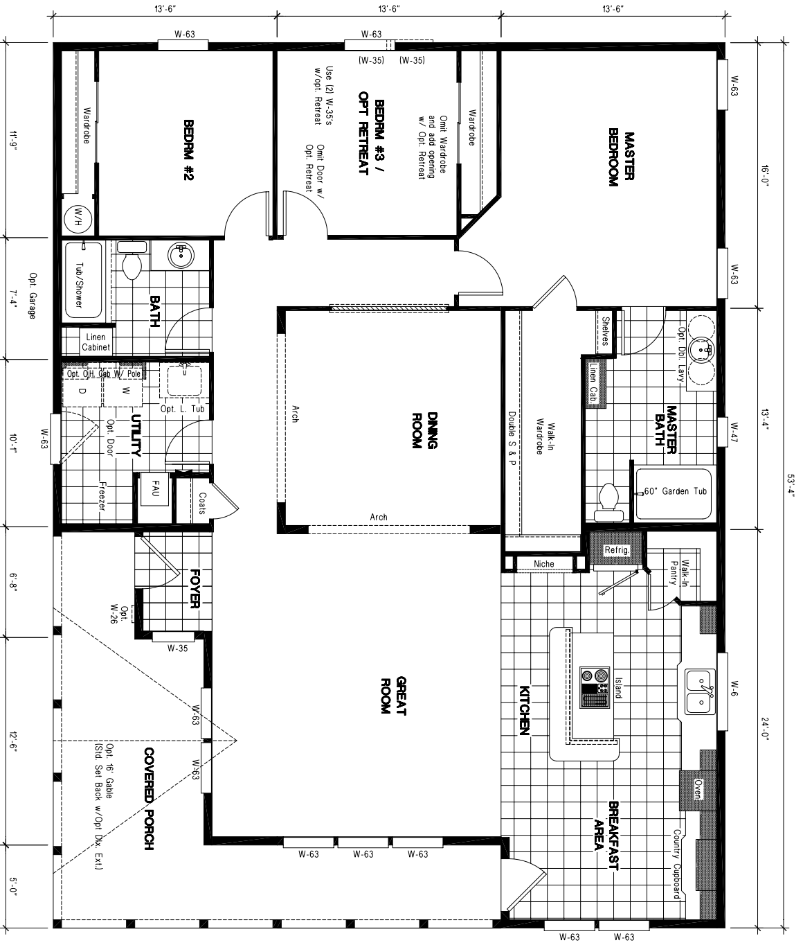
GE 531K THREE BEDROOM, TWO BATH, GREAT ROOM 1879 SQ. FT.
