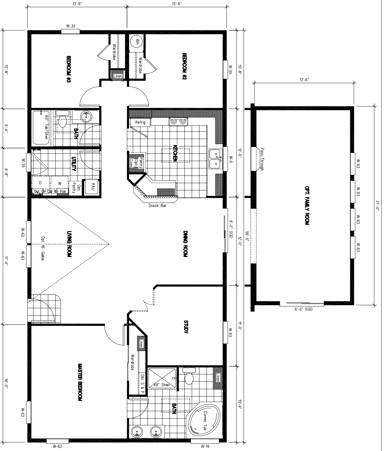
GE 567F THREE BEDROOM, TWO BATH, OPT. TRANSVERSE TAG - 1512 SQ. FT.
